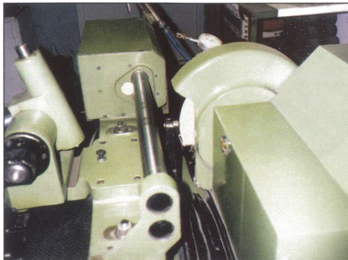
Polishing of the grinding stone
