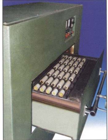
UV irradiation method
